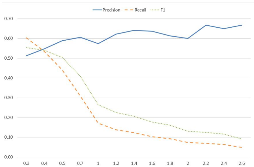
Figure C.1: Query performance for different uncertainty thresholds
