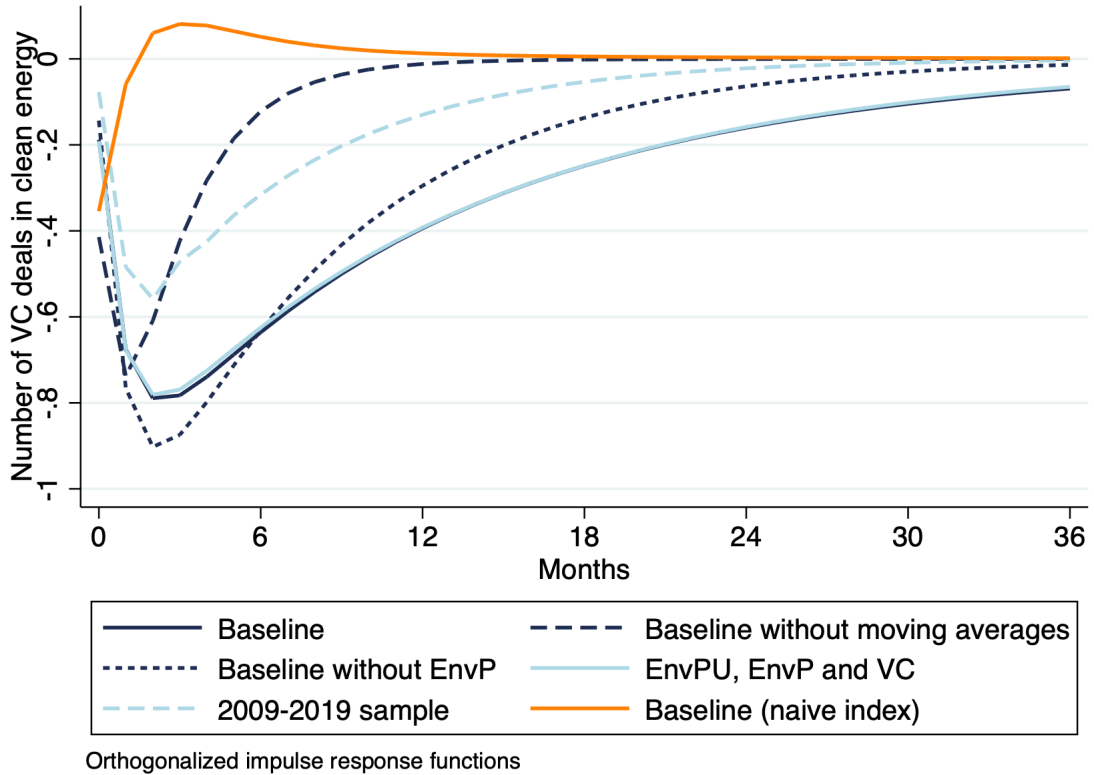
Figure 11: Clean energy venture capital deals responses to EnvPU Shock (IRFs), under alternative specifications and samples.
