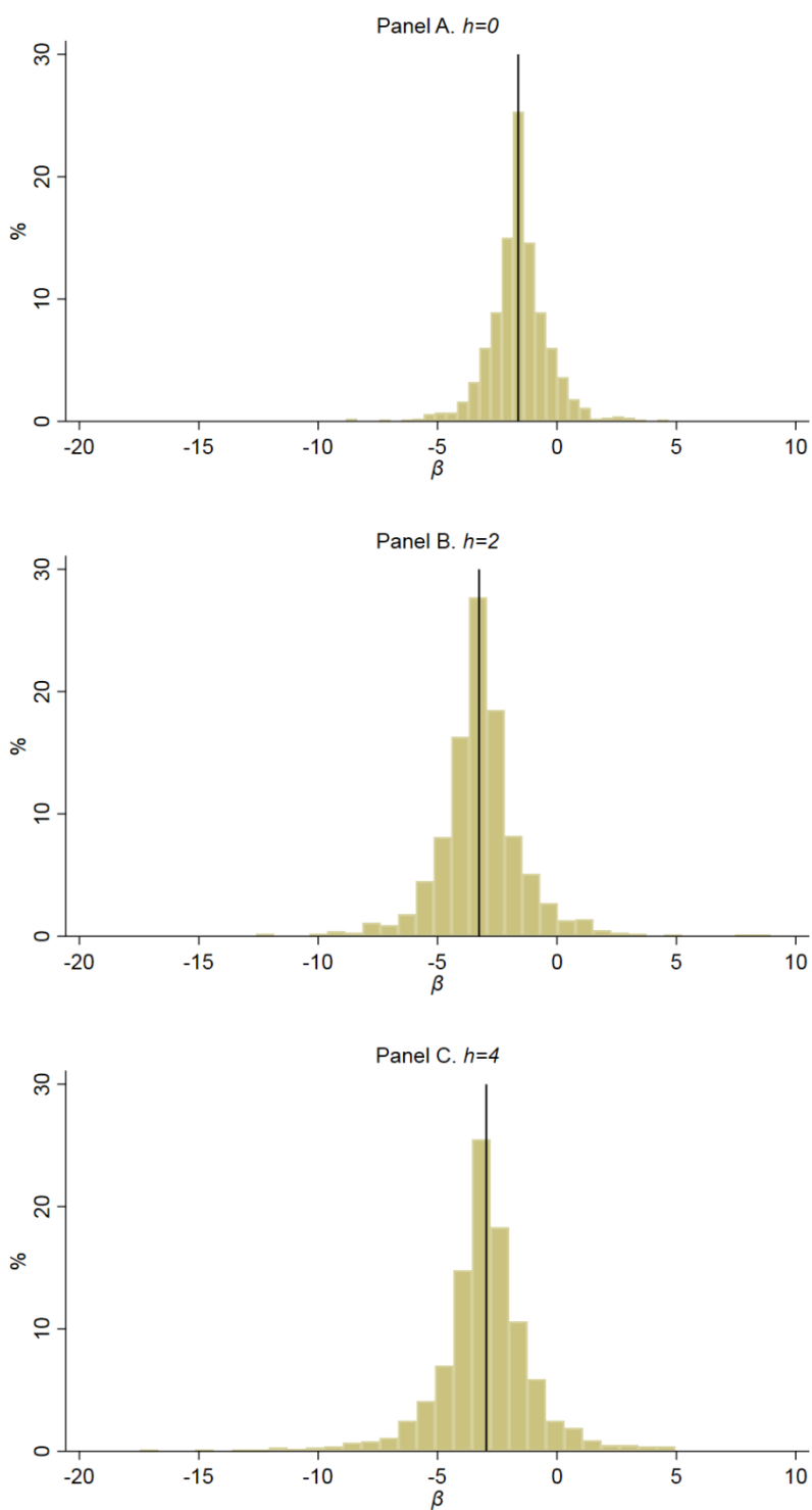
Figure 9. The Distribution of \beta : One-way Reclassification
