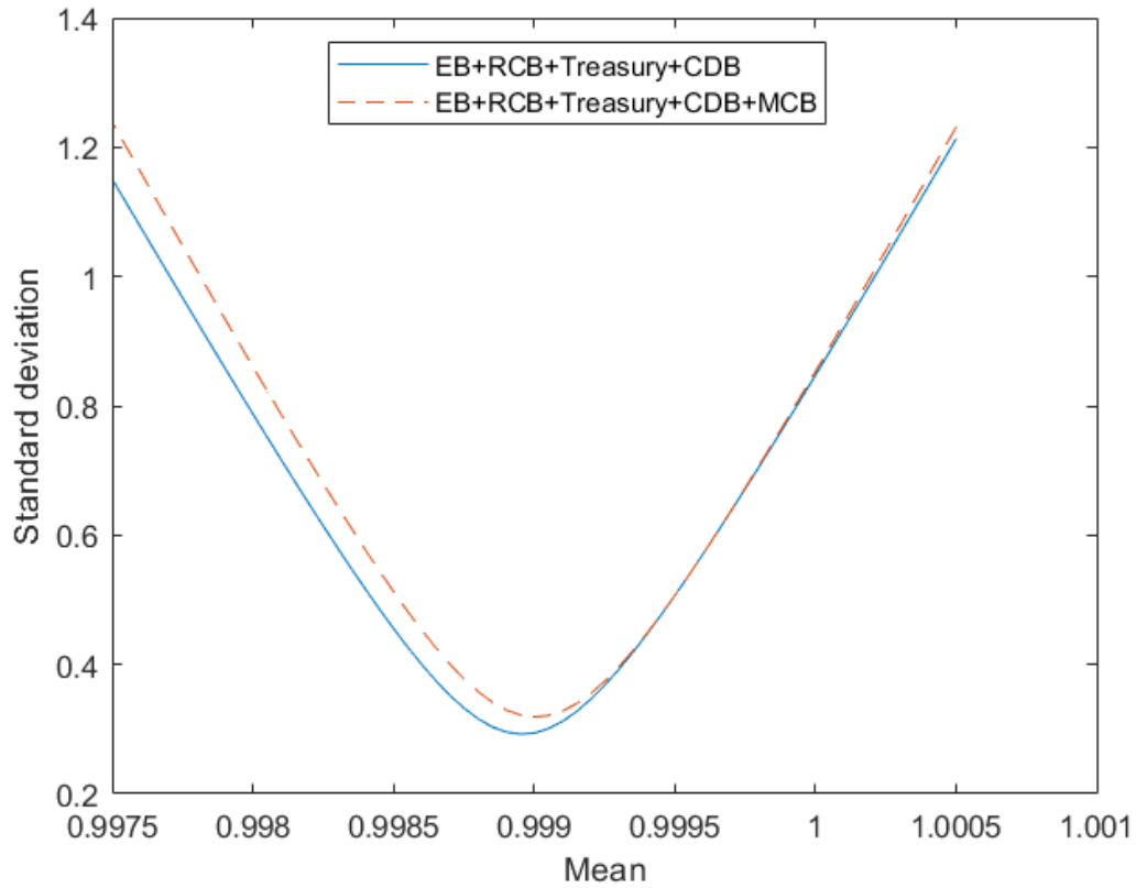
Figure 2. Hansen-Jagannathan bounds.
