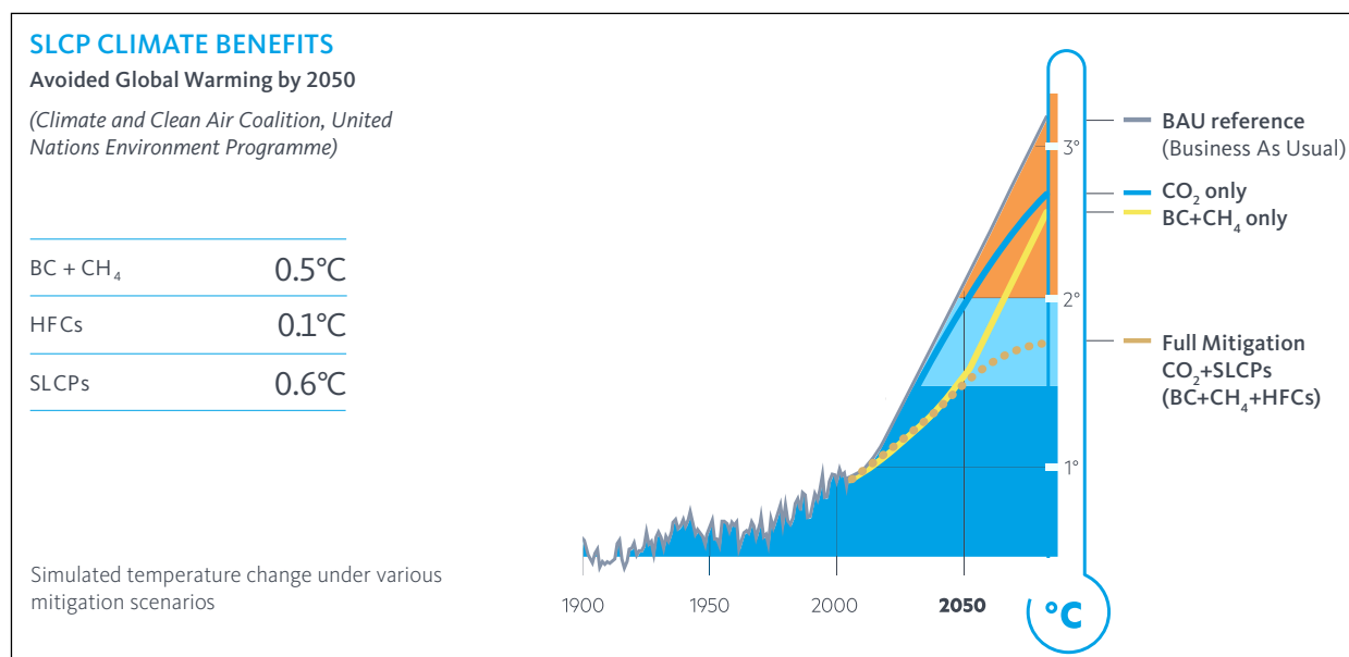
Figure 2: Simulated temperature change under various mitigation scenarios and SLCP Climate benefits.
