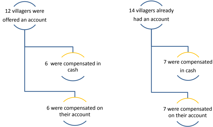
Figure 1: Sampling Strategy
