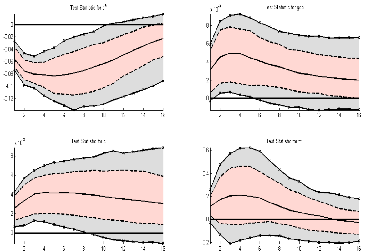
Figure 2: Test - Baseline
