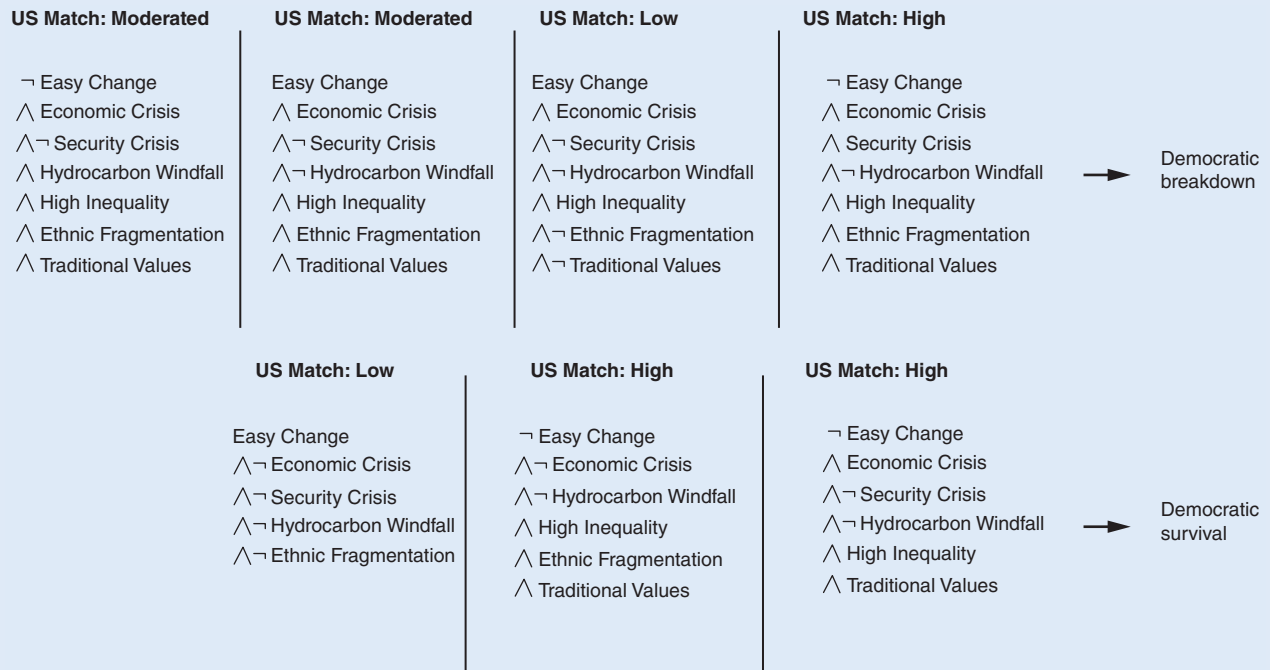
Figure 2 Boolean Reductions
